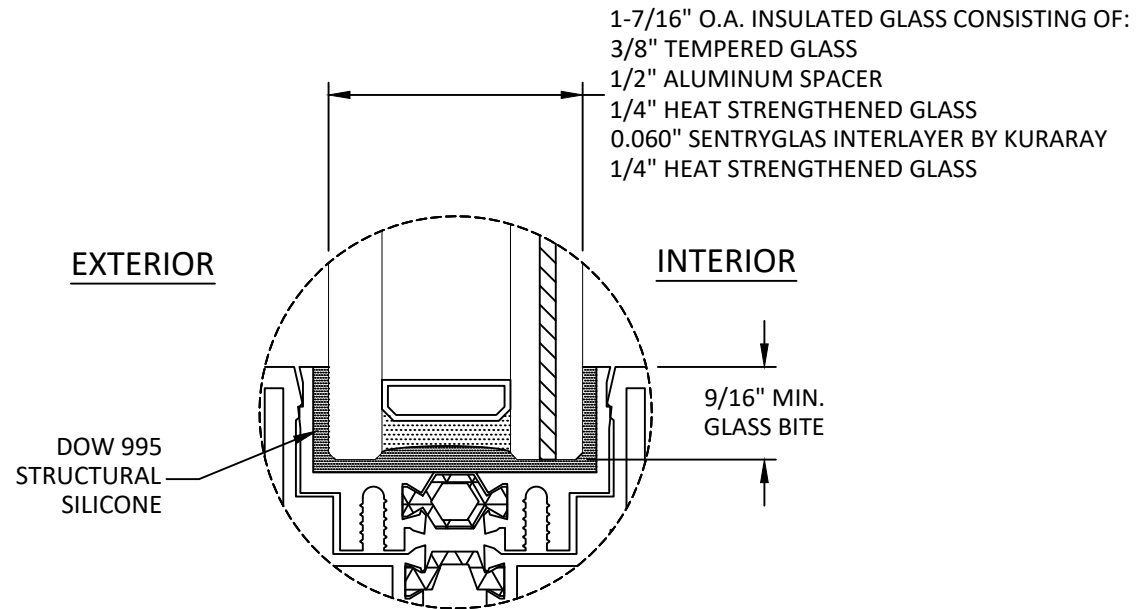
GLAZING DETAIL 1
